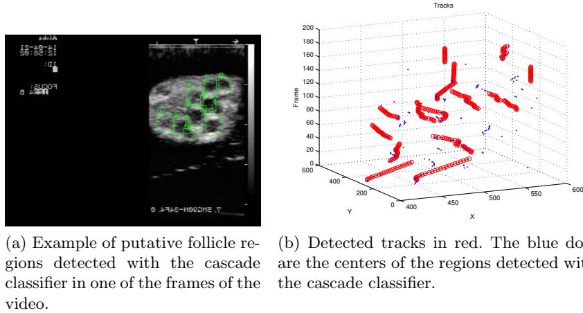
Fig. 2: Follicle-like regions are detected with a cascade classifier. In order to impose temporal coherence, the detections are tracked with multiple Kalman filters.
